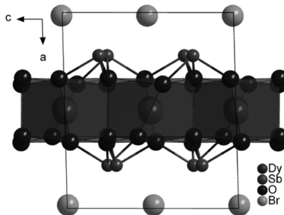
Figure 1 Extended unit cell of DySb_2O_4Br in the monoclinic space group P2_1/c .
