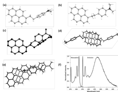
Figure 1 Conformation of molecules in single crystals, a) PyDMA1 and b) PyDMA2. c) Molecular superposition of PyDMA1 (black) and PyDMA2 (red) on pyrene ring with RMSD=0.0427Å. The extent of overlap between the pyrene rings belong to the symmetry related/unit translated molecules in PyDMA1/PyDMA2 in single crystals are 67% and 17%, respectively. f) Absorption (blue) and emission (red) spectra of PyDMA1, in toluene, at 0.1mM concentration.
