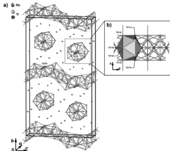
Figure 1 a) Unit cell of the basic structure of \text{Rb}_4\text{Ti}_{13} . The thallium atoms refined with a saw-tooth function in the final model (Ti(19) and Ti(29)) are represented as blue spheres. All remaining atomic positions are shown as red (Rubidium) resp. green (Thallium) ellipsoids (Probability: 90%). b) Detailed view of one chain of interpenetrating icosahedra with 90% probability ellipsoids and atomic labels from the model of the basic structure (projection along [001] ).
