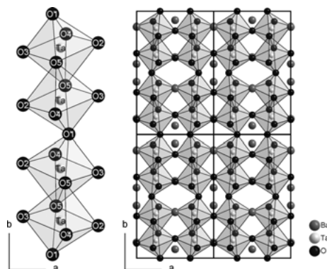
Figure 1 Chains of corner- and edge-sharing [\text{TaO}_6]^{7-} octahedra running along [010] (left) and corrugated layers of these vertex-connected chains parallel to the (001) plane (right) in \text{BaTa}_2\text{O}_6 .
