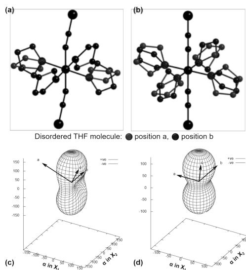
Figure 1 Octahedral coordination of \text{Mg}^{2+} with \text{SCN}^- and THF for a) \alpha\text{-Mg}(\text{SCN})_2 \cdot 4 \text{THF} ; b) \beta\text{-Mg}(\text{SCN})_2 \cdot 4 \text{THF} . Plots showing the variation of the thermal expansion coefficient \alpha with the principal directions X_1 , X_2 and X_3 of c) \alpha\text{-Mg}(\text{SCN})_2 \cdot 4 \text{THF} , d) \beta\text{-Mg}(\text{SCN})_2 \cdot 4 \text{THF} .
