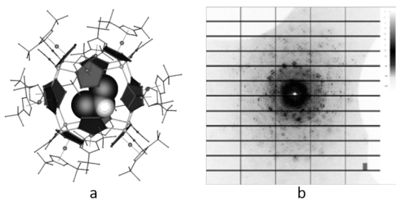
Figure 1 a) Giant cationic supramolecule [(\text{Cp}^*\text{Fe}(\eta^5\text{-P5})_{12}(\text{CuNCCH}_3)_8]^{8+} with an external diameter of 2.5 nm [4]. Hydrogen atoms are omitted for clarity; b) the diffraction pattern from the single crystal at P11 beamline ( E = 18 \text{ keV} , 0.1^\circ scan)
