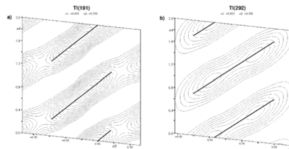
Figure 2 De Wolff's sections from the final structure of \text{Rb}_4\text{Ti}_{13} . a) x_3 - x_4 -section at the Ti(191) site. b) x_3 - x_4 -section at the Ti(292) site (Contour lines at intervals of 30\ \text{e}^- \times 10^{-6}\text{pm}^{-3} ). The difference between the atomic labels of the final and the basic structure (Fig.1) results from the symmetry reduction from Cmca to Pbcm . The Ti(19) site splits up to Ti(191) and Ti(192) and the Ti(29) site splits up to Ti(291) and Ti(292).
