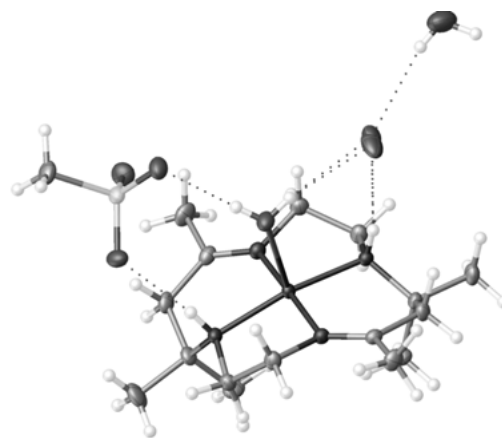
Figure 1 IAM ( ShelXL ): R = 0.0404 , r.m.s.\Delta\rho 0.089, \max/\min \Delta\rho 0.59/-0.34; C-C bond error 0.0017-0.0020 Å; IAM+correction ( ShelXL ): R = 0.036 , r.m.s.\Delta\rho 0.081, \max/\min \Delta\rho 0.40/-0.34; C-C bond error 0.0016-0.0017 Å; NoSpherA2 ( ORCA , def2-TZVPD ): R = 0.036 , \max/\min \Delta\rho 0.7/-0.6, C-C bond error 0.0015-0.0018 Å.
