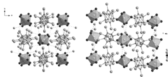
Figure 2 Simplified network {}^3_{\infty}[[\text{Mn}(\text{H}_2\text{O})_6](\text{H}_2\text{O})_{6/2}]^{2+} of water-bridged [\text{Mn}(\text{H}_2\text{O})_6]^{2+} octahedra in \text{Mn}(\text{H}_2\text{O})_6[\text{B}_{10}\text{Cl}_{10}] \cdot 2.5 \text{H}_2\text{O} .
