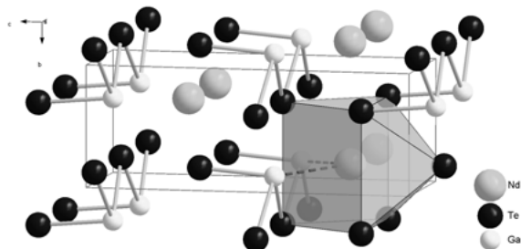
Figure 1 Unit cell of \text{NdGaTe}_2 in which the polyanionic substructure has been highlighted. The Nd-Ga contacts are shown by dashed “bonds”.
