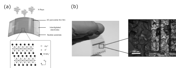
Figure 1 (a) Schematic of the device structure. Bottom: graphical representation of the (R - NH_3)_2PbX_4 crystal structure projected along the direction \langle 010 \rangle showing the stacking of the 2D layers. (b) Photograph (left) and microscope image (right) showing the crystal grains morphology close to the pixel area.
